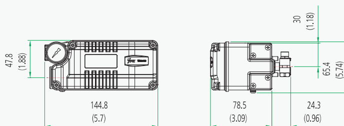
Dimensions: mm (Inches *)
