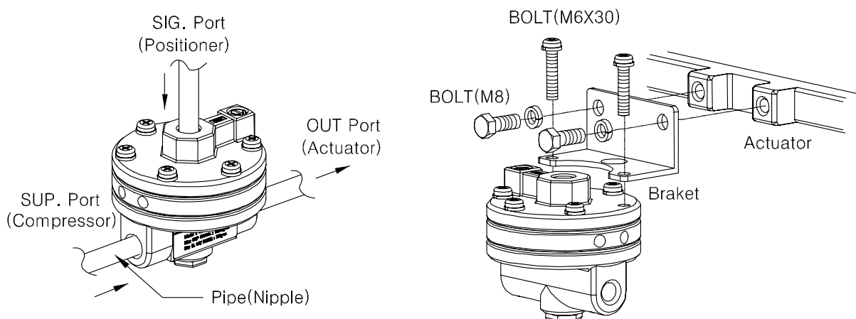
Fig. 3-1: How to install volume booster
