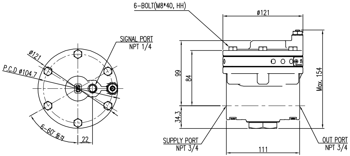
Fig. 2-6: YT-310 / 315 dimension
