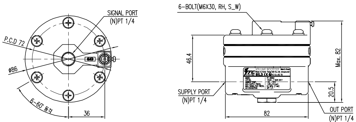
Fig. 2-5: YT-300 / 305 dimension
