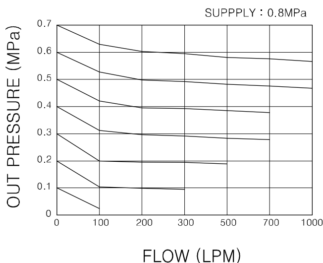
Fig. 2-10: YT-320 / 325
